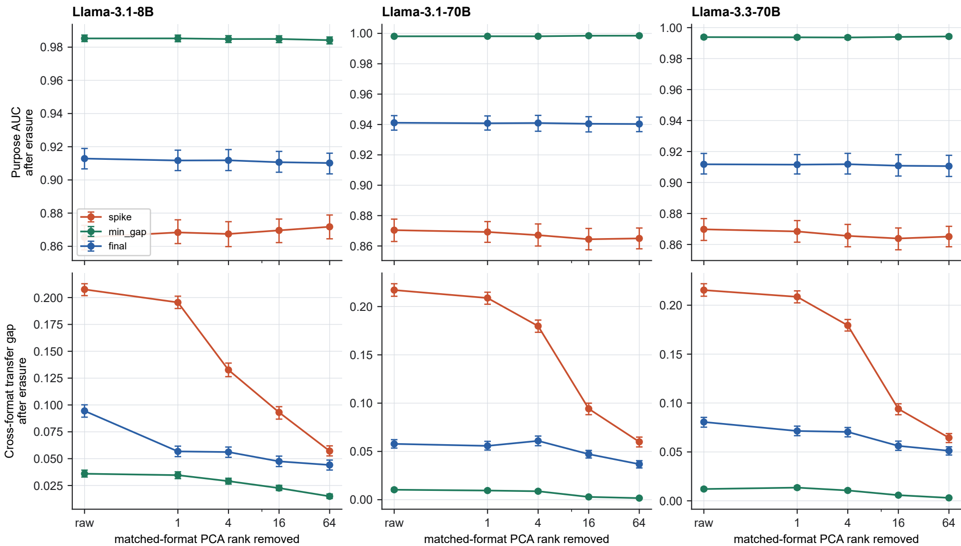
Transfer gap collapses with matched-format rank; purpose AUC stays flat (error bars: payload-block-bootstrap 95% CI, N=1000)
