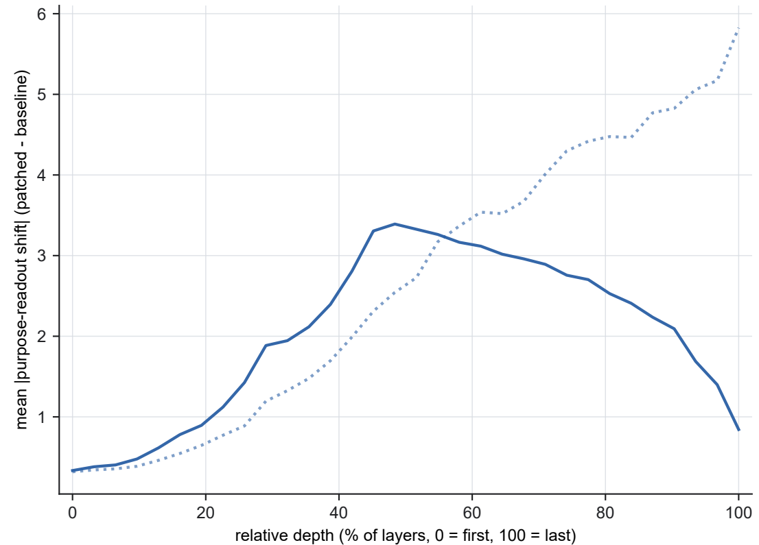
Purpose-readout disruption: real_swap vs. matched_control
