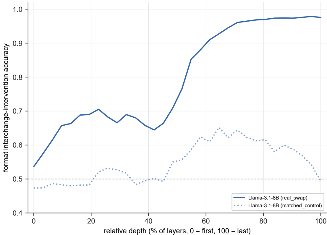
Format readout follows real_swap, not matched_control
