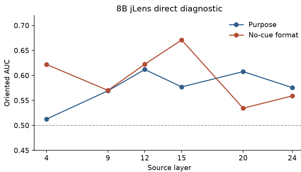
Figure 5: Development-only 8B Jacobian-lens direct diagnostic.
