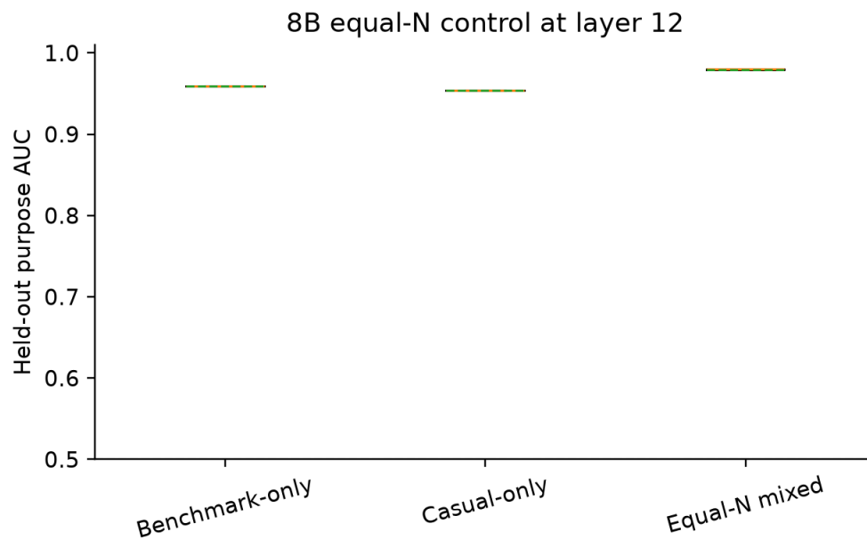
Figure 4: Four-seed 8B equal-training-size control at layer 12. This is not an all-model replication.
