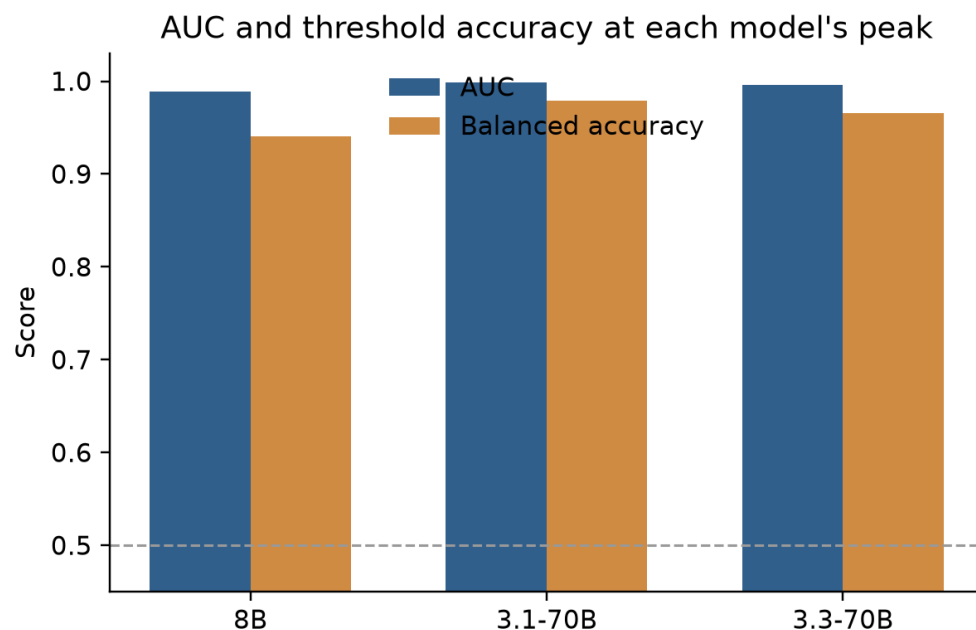
Figure 3: AUC and balanced accuracy at descriptive peaks.
