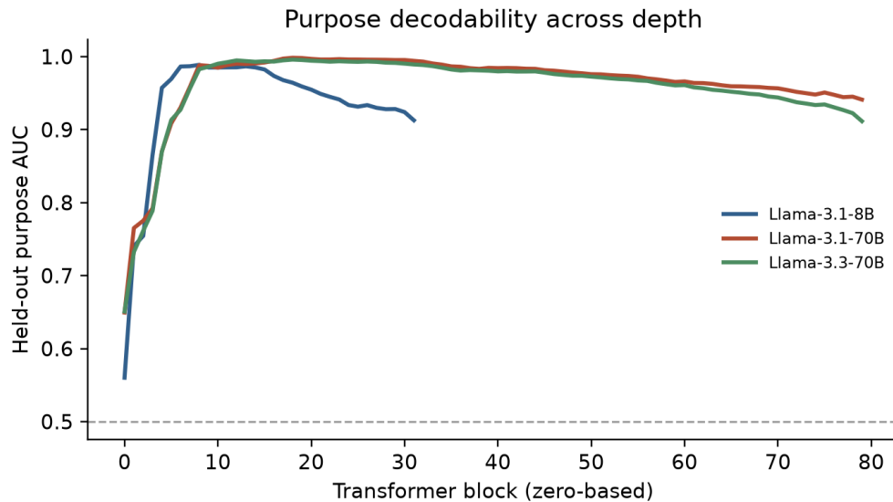
Figure 1: Held-out purpose AUC across depth for the three pinned model result files.
