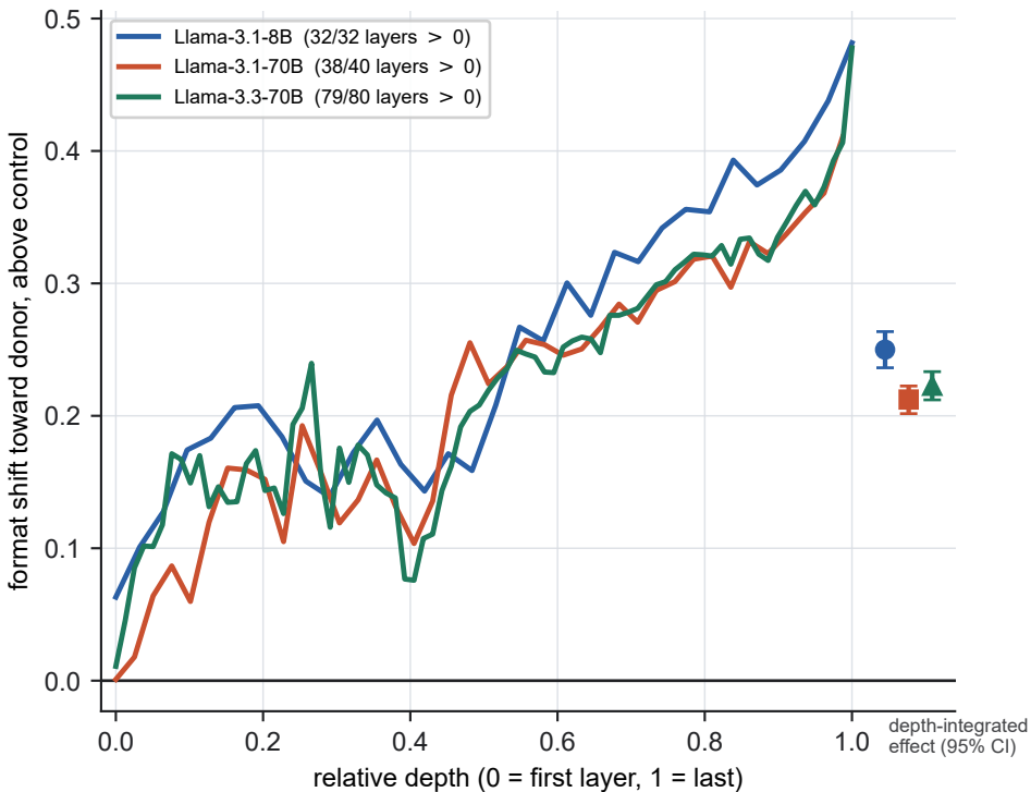
A. The swap moves the format readout, at nearly every layer
