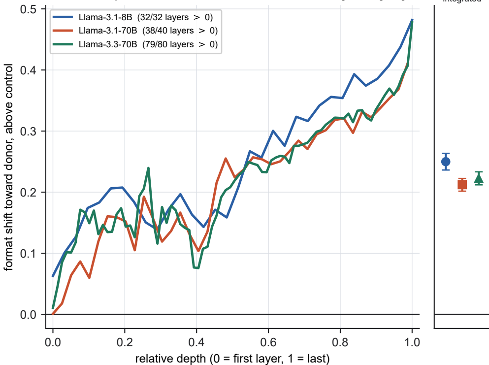
A. The swap moves the format readout, at nearly every layer
