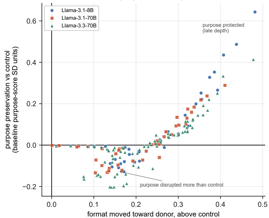
B. Format is carried, purpose is not spared
