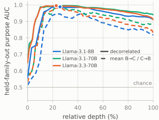
A Single-format transfer by depth
