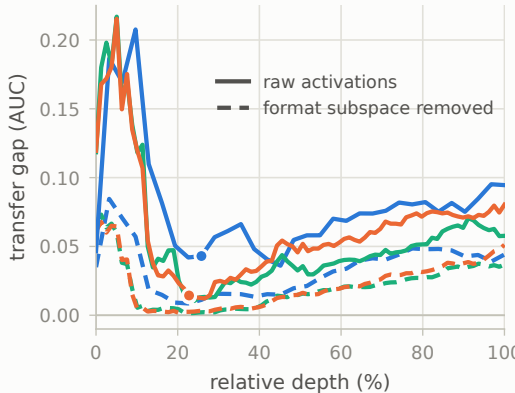
B Gap, raw vs. rank-64 projected
