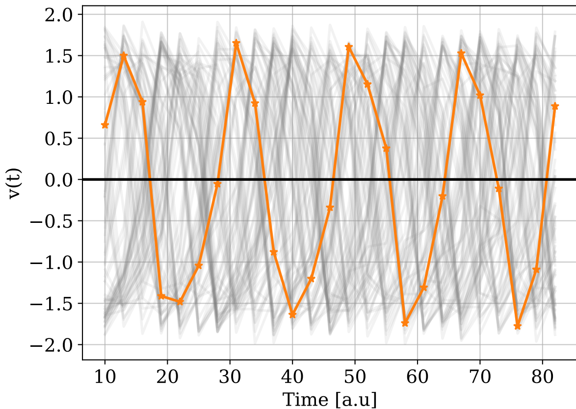
Class 1: b=1.175
