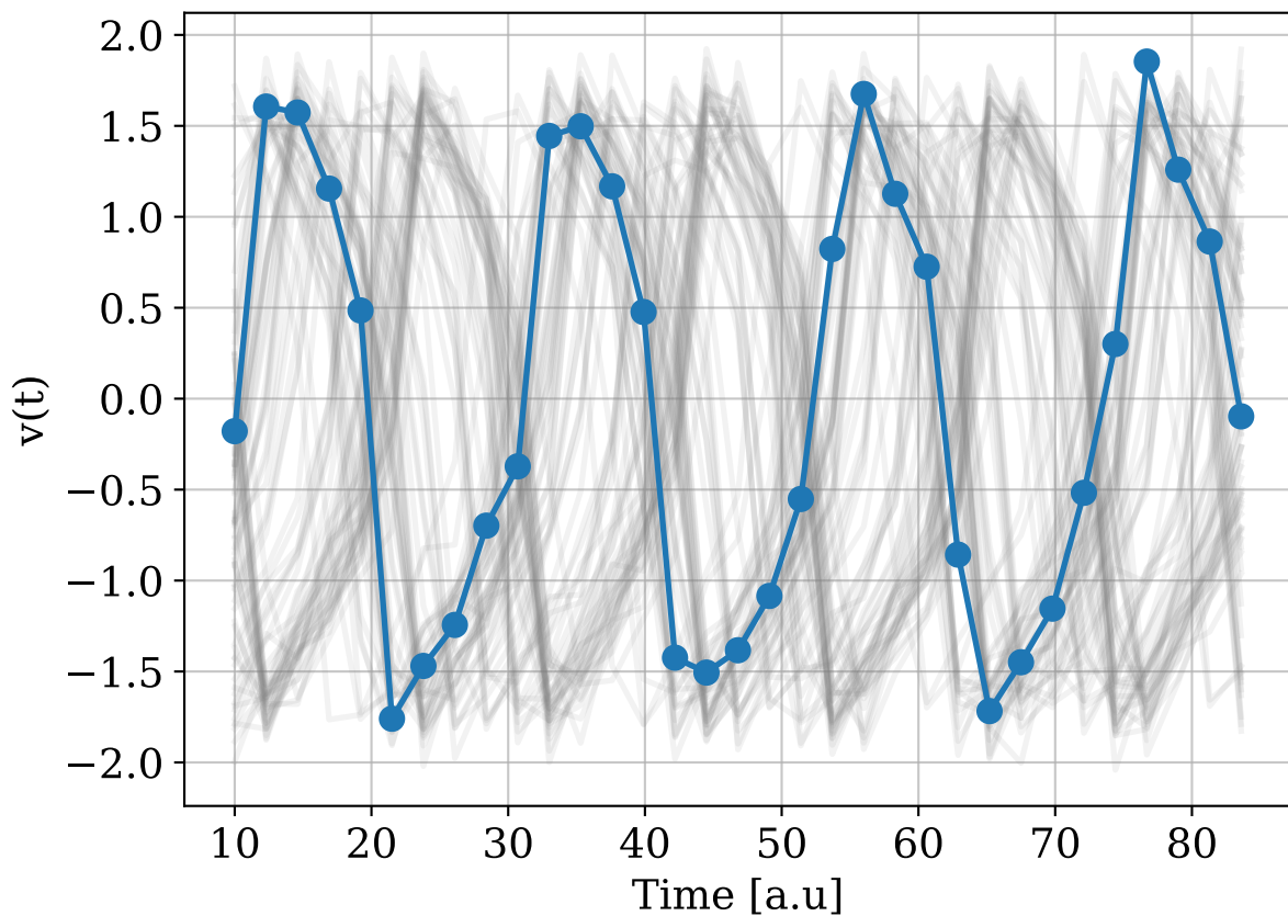
Class 0: b=1.0
