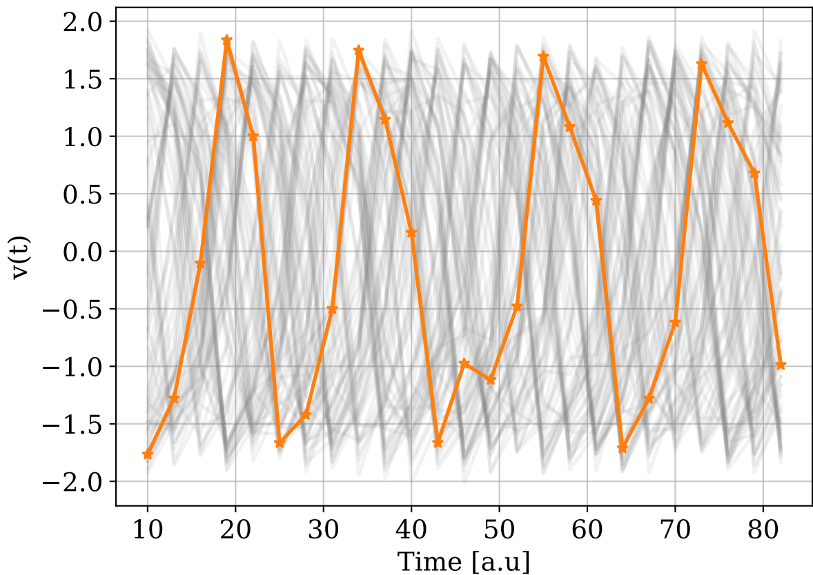
Class 1: b=1.175
