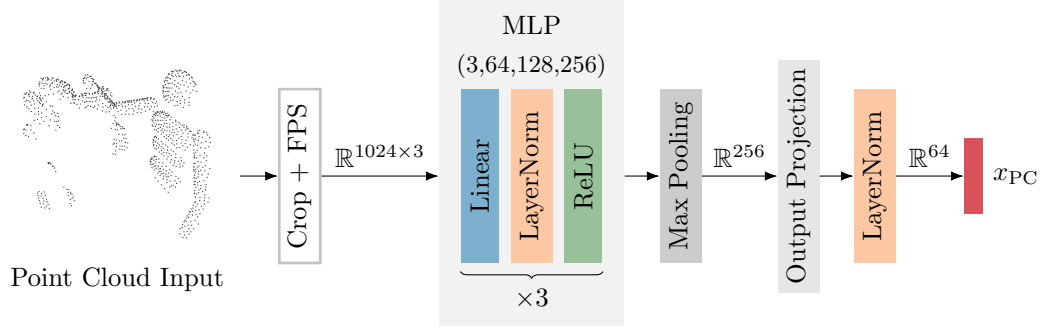
Figure 2: 3D Point Cloud Encoder [2].
