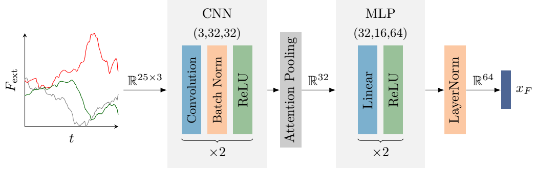
Figure 1: Force history encoder.
