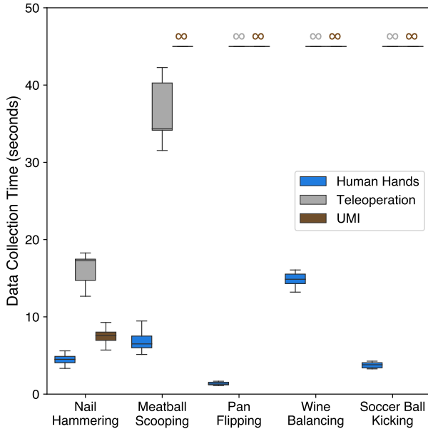
Fig. 11: Quantitative Comparison of Data Collection Methods. Human hands significantly reduce data collection time—by 73% for nail hammering and 81% for meatball scooping—while maintaining consistently low variation across trials. Teleoperation fails entirely in dynamic tasks and tasks requiring high precision. In nail hammering, human hands are 41% faster than UMI [11], which also struggles in dynamic scenarios and low-texture environments.
