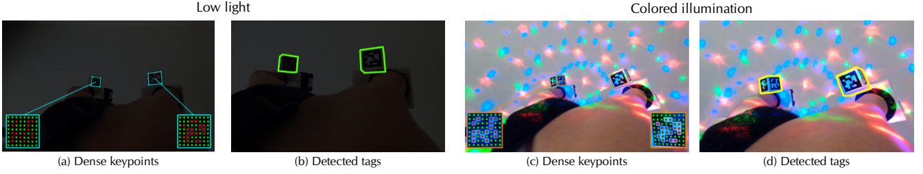
Fig. S2. Qualitative lighting robustness of fiducial detection. (a,b) Low-light examples. (c,d) Examples with spatially varying colored illumination. For each condition, the left panel shows dense keypoints with enlarged tag-grid insets, and the right panel shows detected tag outlines. All detection overlays are preserved from the original images.
