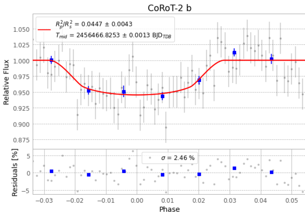
Figure 1 — FinalLightCurve_CoRoT-2 b_2013-06-22.png (SHA-256 39eb07bc2182b27d...)
