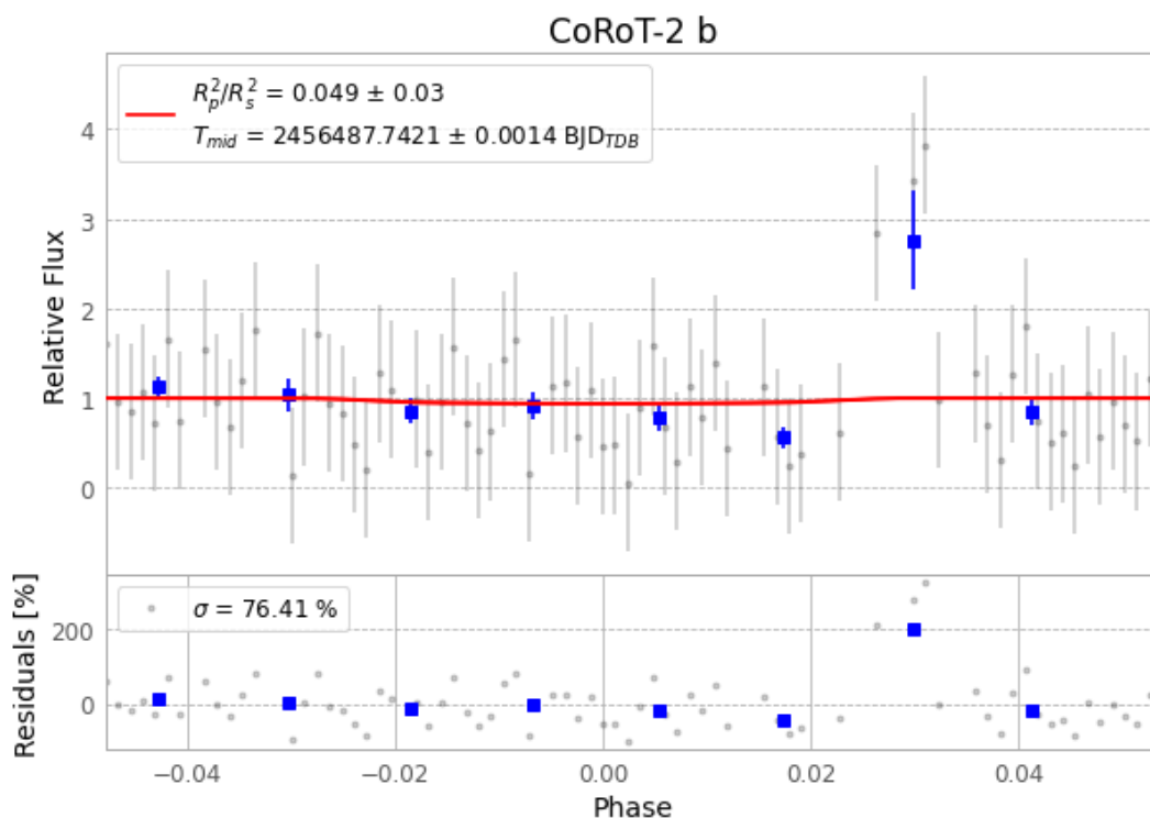
Figure 1 — FinalLightCurve_CoRoT-2 b_2013-07-13.png (SHA-256 833770a85f4cda85...)
