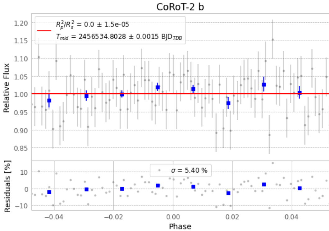
Figure 1 — FinalLightCurve_CoRoT-2 b_2013-08-29.png (SHA-256 8ed71d11d75deeab...)
