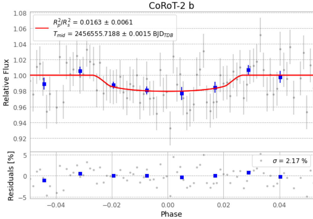
Figure 1 — FinalLightCurve_CoRoT-2 b_2013-09-19.png (SHA-256 bf20c81227d89406...)
