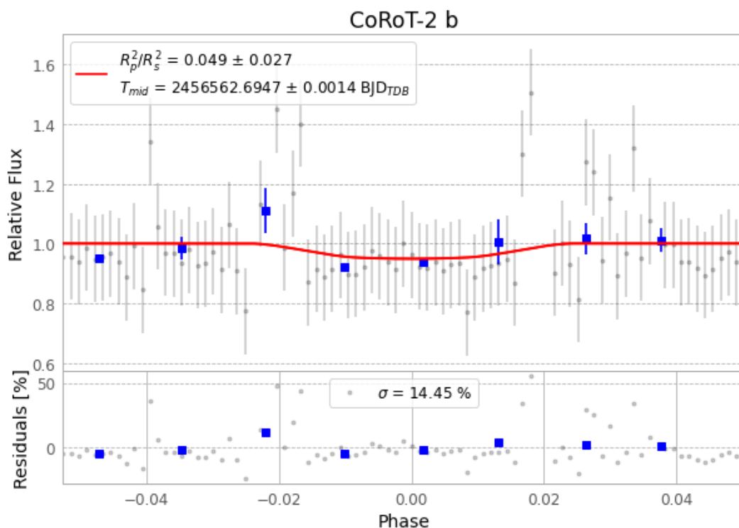
Figure 1 — FinalLightCurve_CoRoT-2 b_2013-09-26.png (SHA-256 106cf96c23ed7f4f...)
