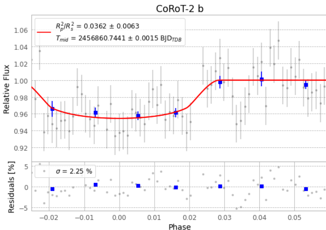
Figure 1 — FinalLightCurve_CoRoT-2 b_2014-07-21.png (SHA-256 a9c2e7e7286b2492...)
