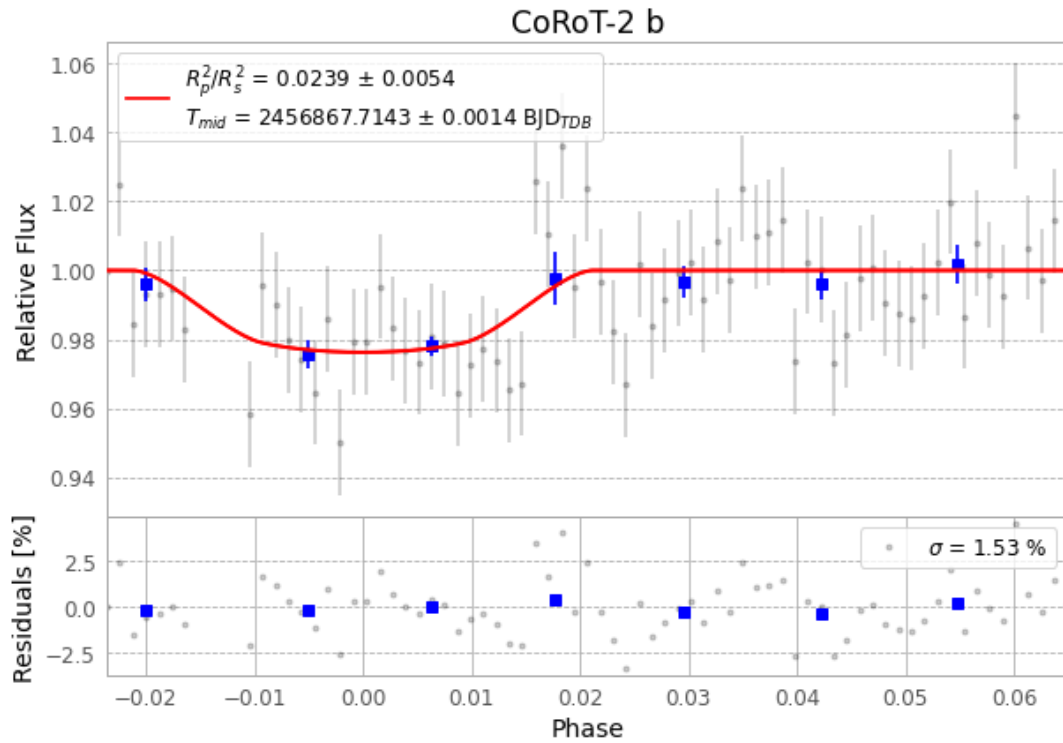
Figure 1 — FinalLightCurve_CoRoT-2 b_2014-07-28.png (SHA-256 3bb98b1f92cd9027...)
