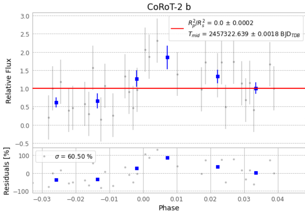
Figure 1 — FinalLightCurve_CoRoT-2 b_2015-10-26.png (SHA-256 1ab3617f54d6513f...)
