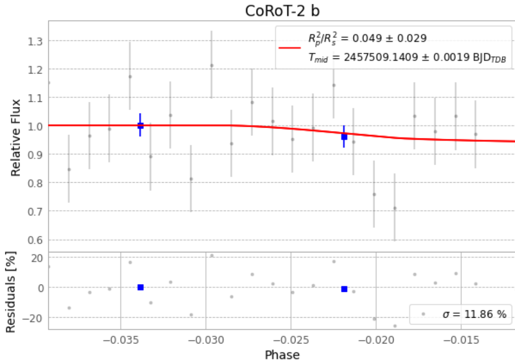
Figure 1 — FinalLightCurve_CoRoT-2 b_2016-05-02.png (SHA-256 070e531d869f7849...)
