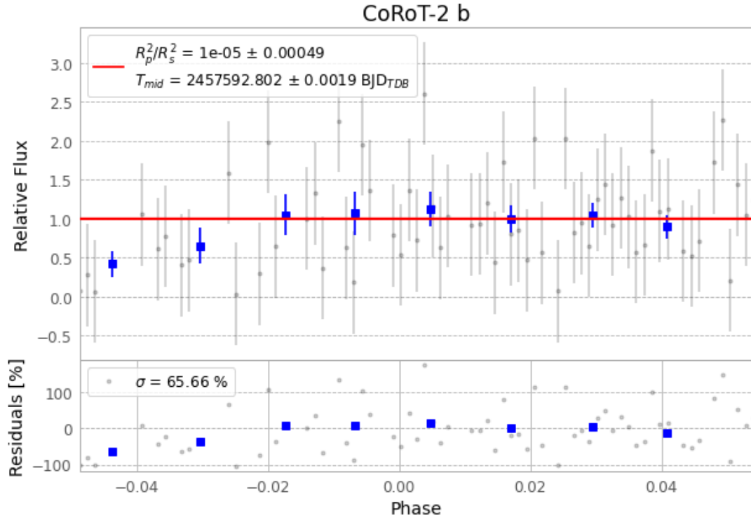
Figure 1 — FinalLightCurve_CoRoT-2 b_2016-07-22.png (SHA-256 0c05bd67d01b1121...)
