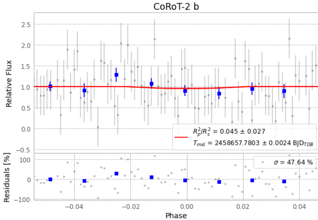
Figure 1 — FinalLightCurve_CoRoT-2 b_2019-06-22.png (SHA-256 f1ac1a49a8f76541...)
