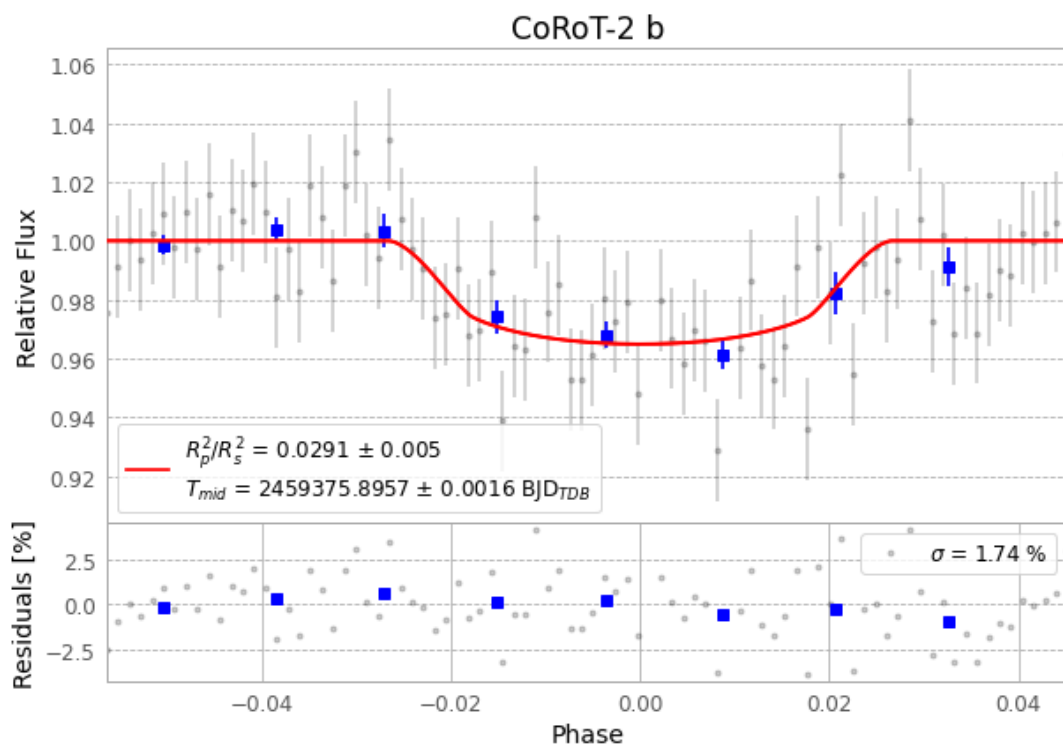
Figure 1 — FinalLightCurve_CoRoT-2 b_2021-06-10.png (SHA-256 eb541bbb32e54313...)
