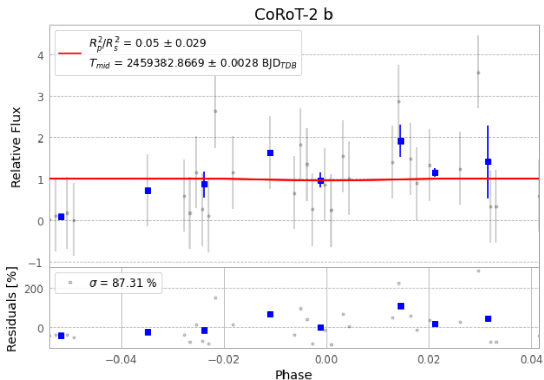
Figure 1 — FinalLightCurve_CoRoT-2 b_2021-06-16.png (SHA-256 c3b186d9076f3b23...)
