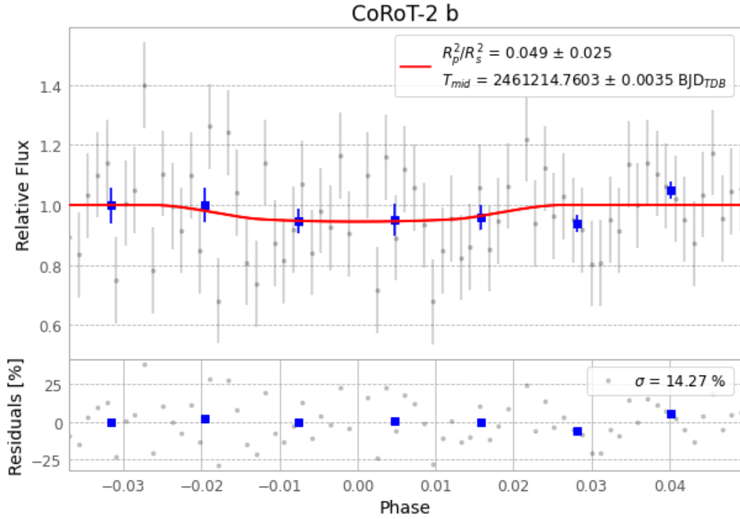
Figure 1 — FinalLightCurve_CoRoT-2 b_2026-06-22.png (SHA-256 59f8a00508572fe0...)
