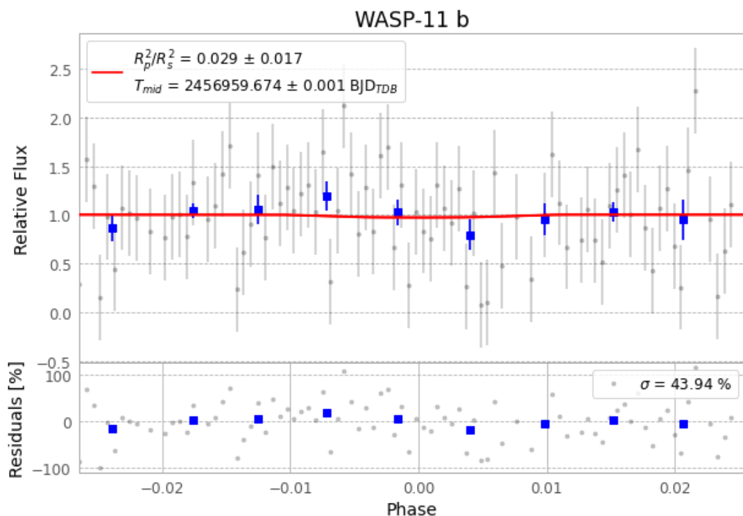
Figure 1 — FinalLightCurve_WASP-11 b_2014-10-28.png (SHA-256 dee6dfe552a86172...)
