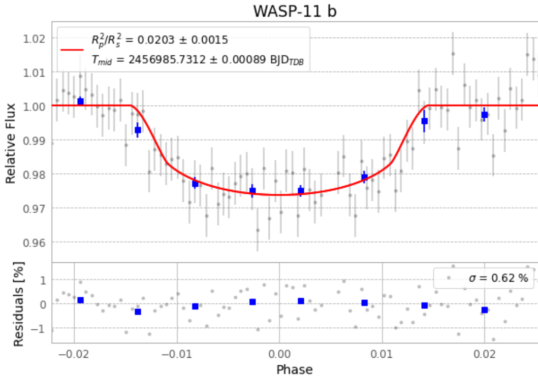
Figure 1 — FinalLightCurve_WASP-11 b_2014-11-23.png (SHA-256 0b8f4da56b3513e6...)
