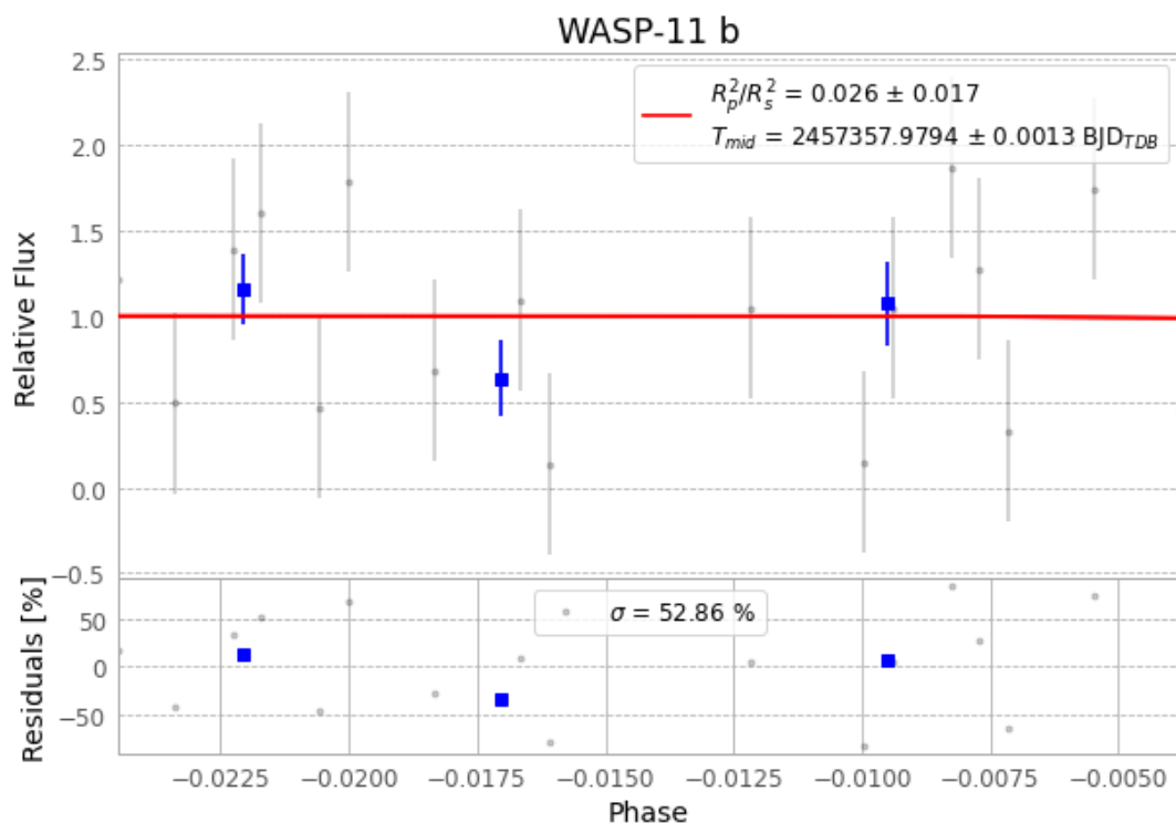
Figure 1 — FinalLightCurve_WASP-11 b_2015-12-04.png (SHA-256 b5381e36943d0654...)
