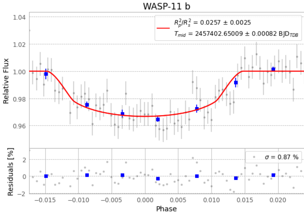
Figure 1 — FinalLightCurve_WASP-11 b_2016-01-14.png (SHA-256 3e8ba068ef666df4...)
