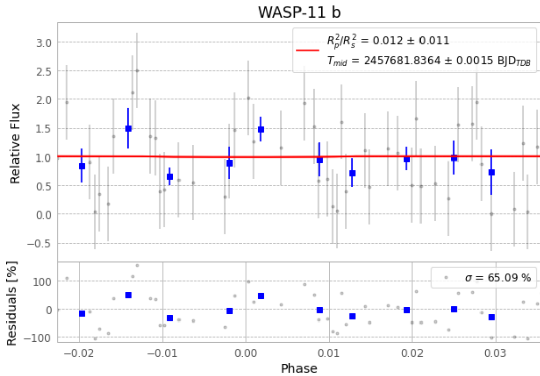
Figure 1 — FinalLightCurve_WASP-11 b_2016-10-19.png (SHA-256 72d8eb8eddd7a196...)
