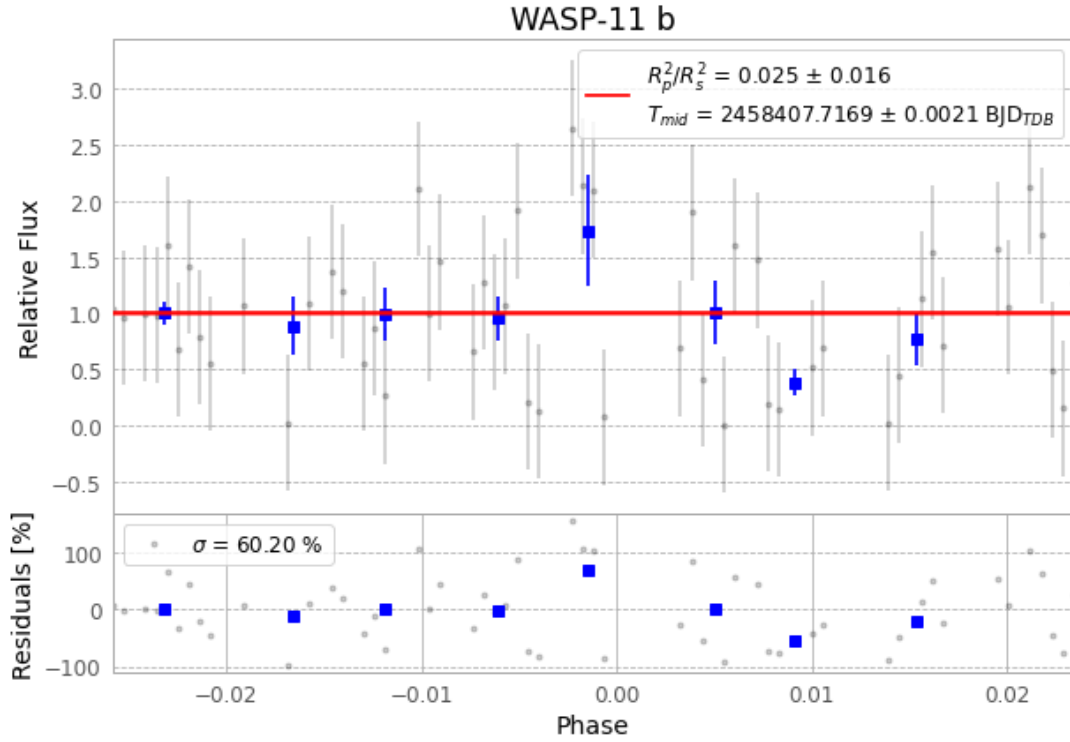
Figure 1 — FinalLightCurve_WASP-11 b_2018-10-15.png (SHA-256 4181e7e5163831b5...)
