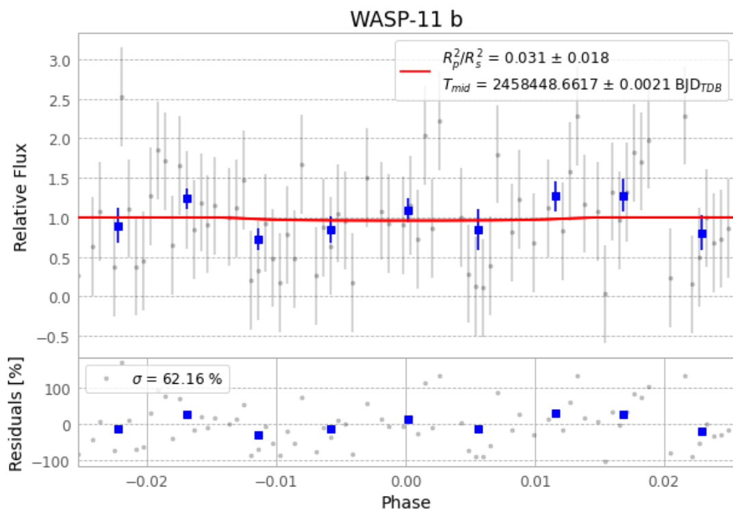
Figure 1 — FinalLightCurve_WASP-11 b_2018-11-25.png (SHA-256 63053b98728071c8...)
