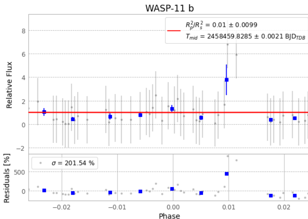
Figure 1 — FinalLightCurve_WASP-11 b_2018-12-06.png (SHA-256 3436c79c64877213...)
