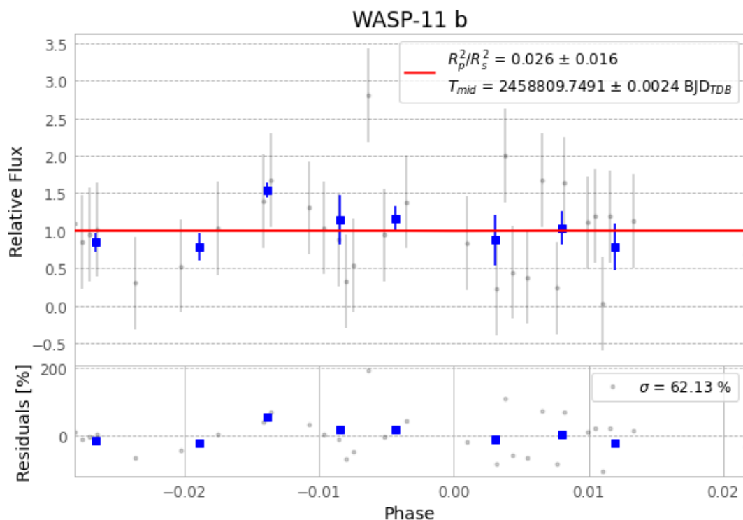
Figure 1 — FinalLightCurve_WASP-11 b_2019-11-21.png (SHA-256 09fa6465c5f75439...)
