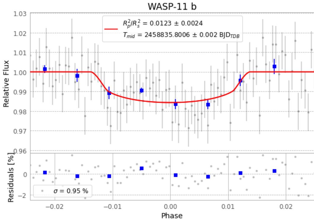
Figure 1 — FinalLightCurve_WASP-11 b_2019-12-17.png (SHA-256 3c10a5e1cf3350d9...)
