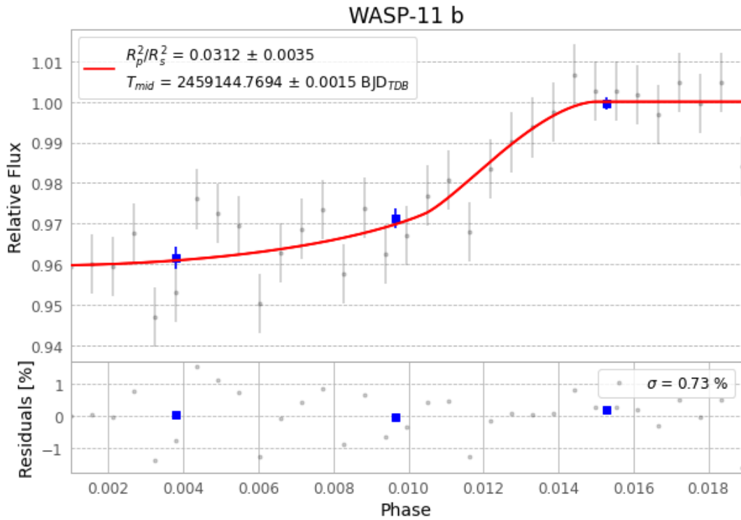
Figure 1 — FinalLightCurve_WASP-11 b_2020-10-21.png (SHA-256 2be3c32e71061d00...)
