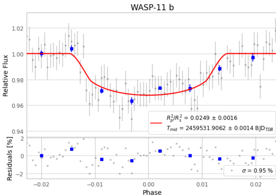
Figure 1 — FinalLightCurve_WASP-11 b_2021-11-13.png (SHA-256 6673ceaaf26ee3c6...)
