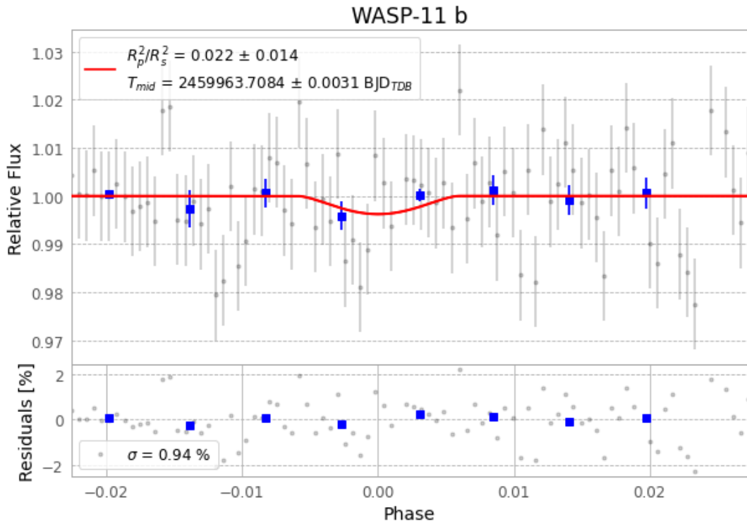
Figure 1 — FinalLightCurve_WASP-11 b_2023-01-18.png (SHA-256 8f55525ed3823a6e...)
