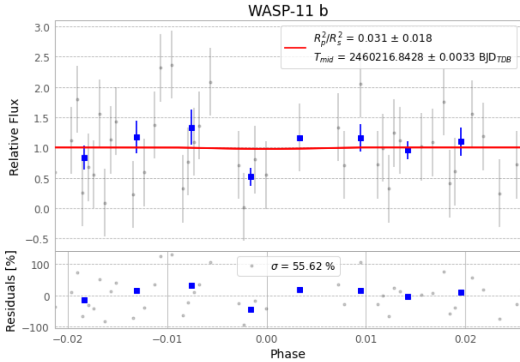
Figure 1 — FinalLightCurve_WASP-11 b_2023-09-28.png (SHA-256 09e7c9a2b58b475b...)
