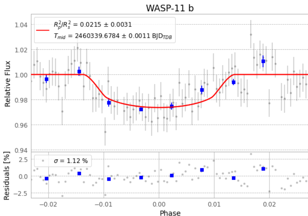
Figure 1 — FinalLightCurve_WASP-11 b_2024-01-29.png (SHA-256 284efeb8237f3e72...)
