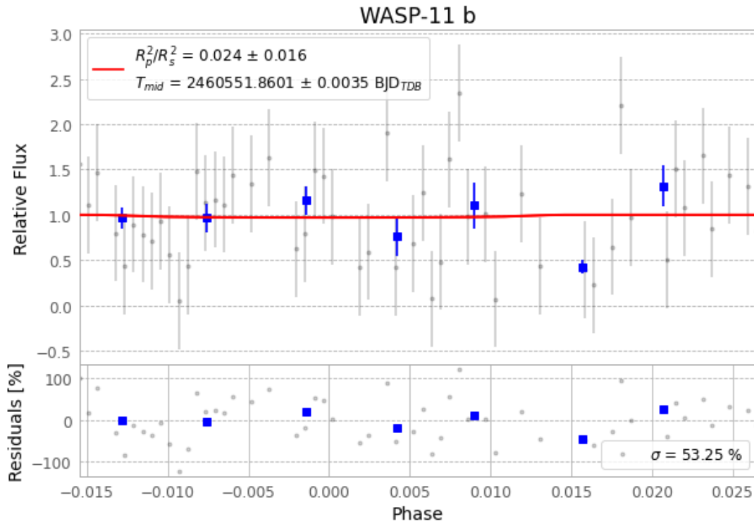
Figure 1 — FinalLightCurve_WASP-11 b_2024-08-29.png (SHA-256 d06f284a8fc456d7...)
