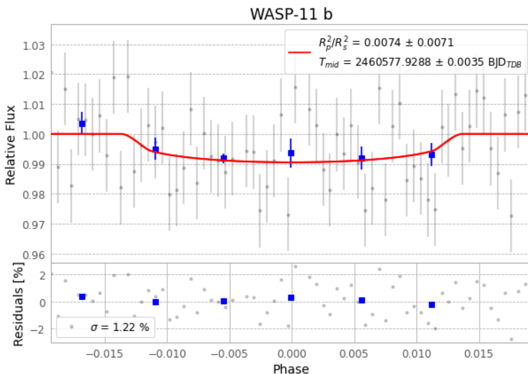
Figure 1 — FinalLightCurve_WASP-11 b_2024-09-24.png (SHA-256 abbad8d7176f0cdc...)
