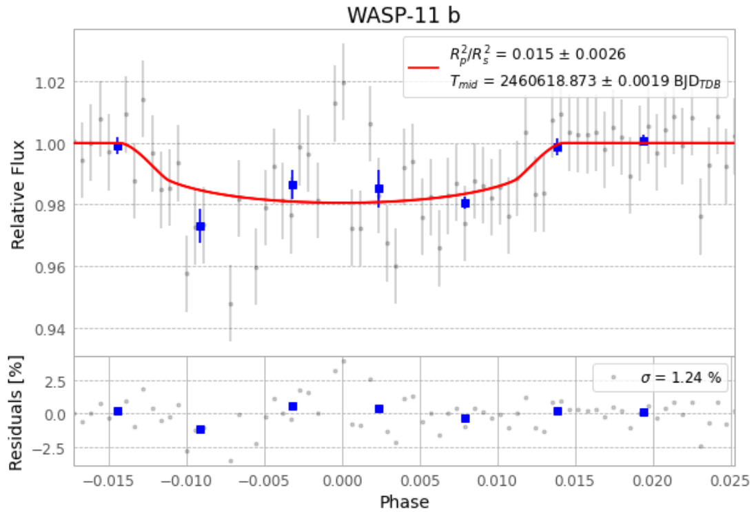
Figure 1 — FinalLightCurve_WASP-11 b_2024-11-04.png (SHA-256 65561e26451a2ad1...)
