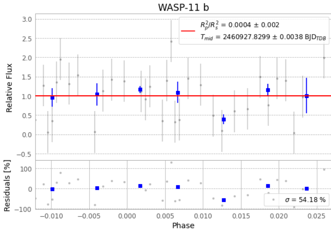
Figure 1 — FinalLightCurve_WASP-11 b_2025-09-08.png (SHA-256 1e066c145f7dd2cc...)
