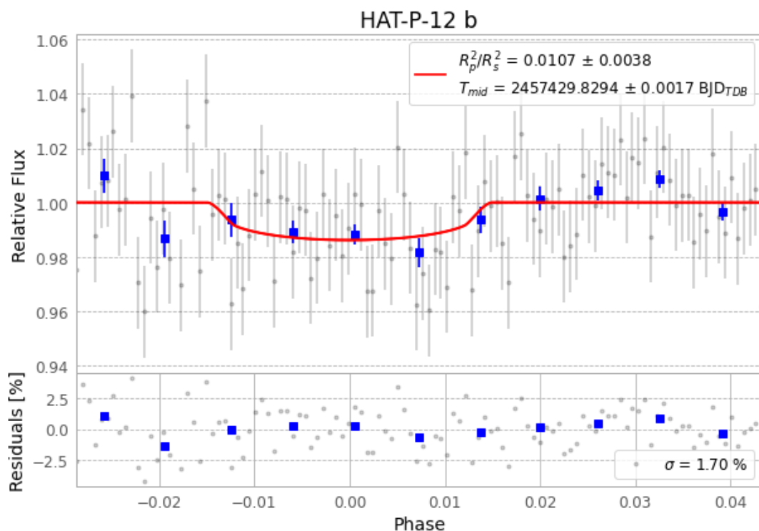
Figure 1 — FinalLightCurve_HAT-P-12 b_2016-02-10.png (SHA-256 5c8137e8f96f43d8...)
