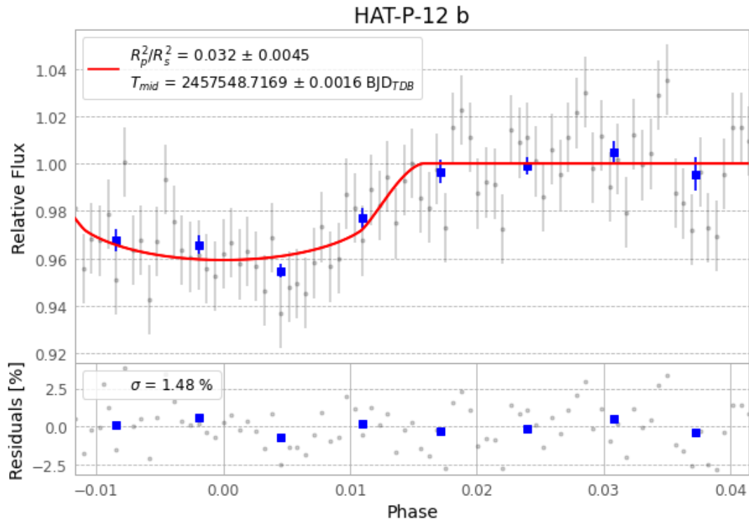
Figure 1 — FinalLightCurve_HAT-P-12 b_2016-06-08.png (SHA-256 aede4f41569efb84...)
