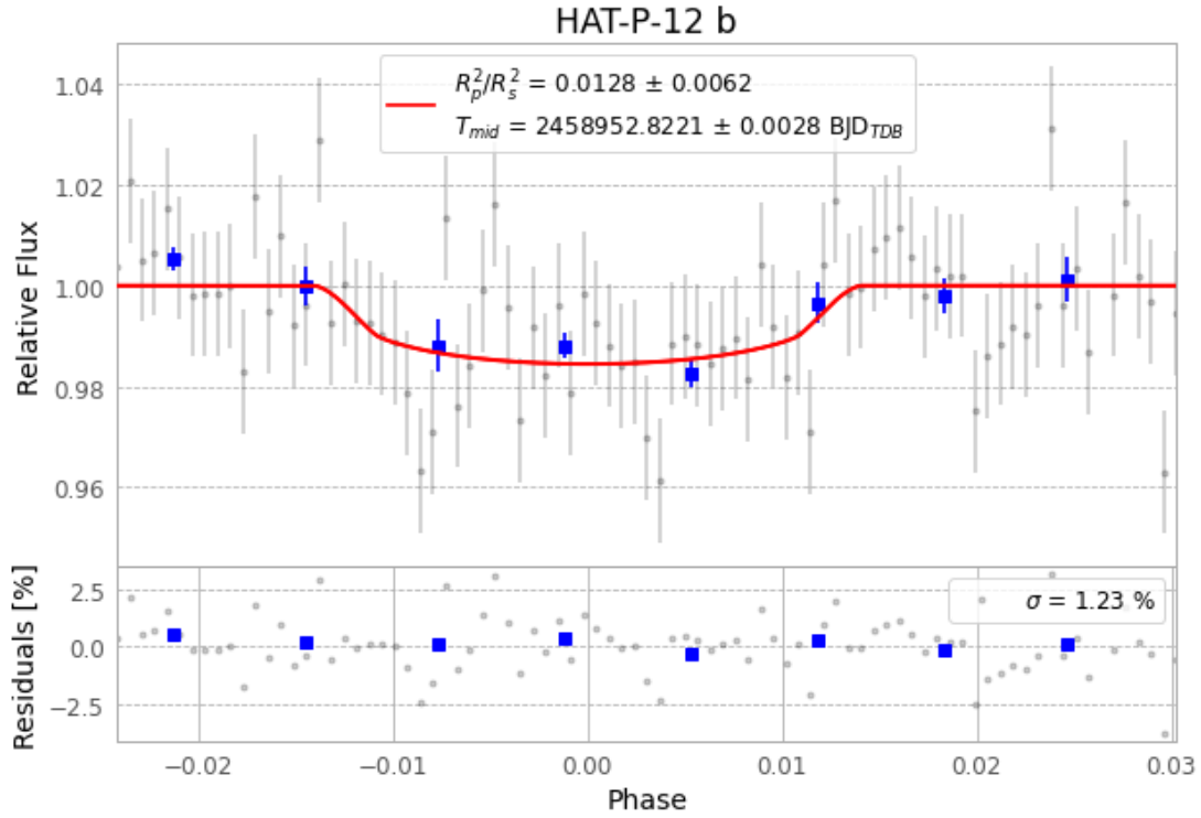
Figure 1 — FinalLightCurve_HAT-P-12 b_2020-04-12.png (SHA-256 082458d99ea0c532...)
