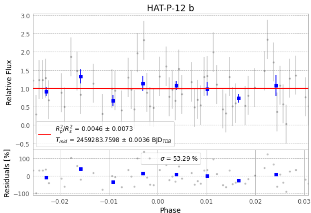
Figure 1 — FinalLightCurve_HAT-P-12 b_2021-03-09.png (SHA-256 9cc96909fbde1ba5...)
