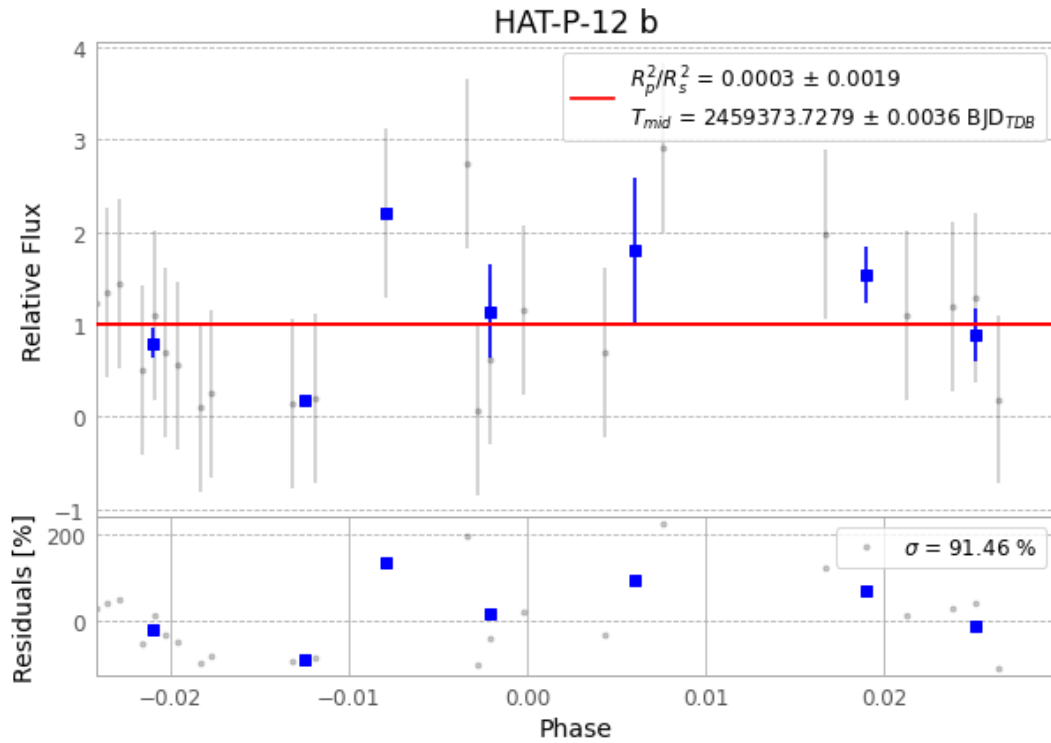
Figure 1 — FinalLightCurve_HAT-P-12 b_2021-06-07.png (SHA-256 b0daf5ac0442716f...)
