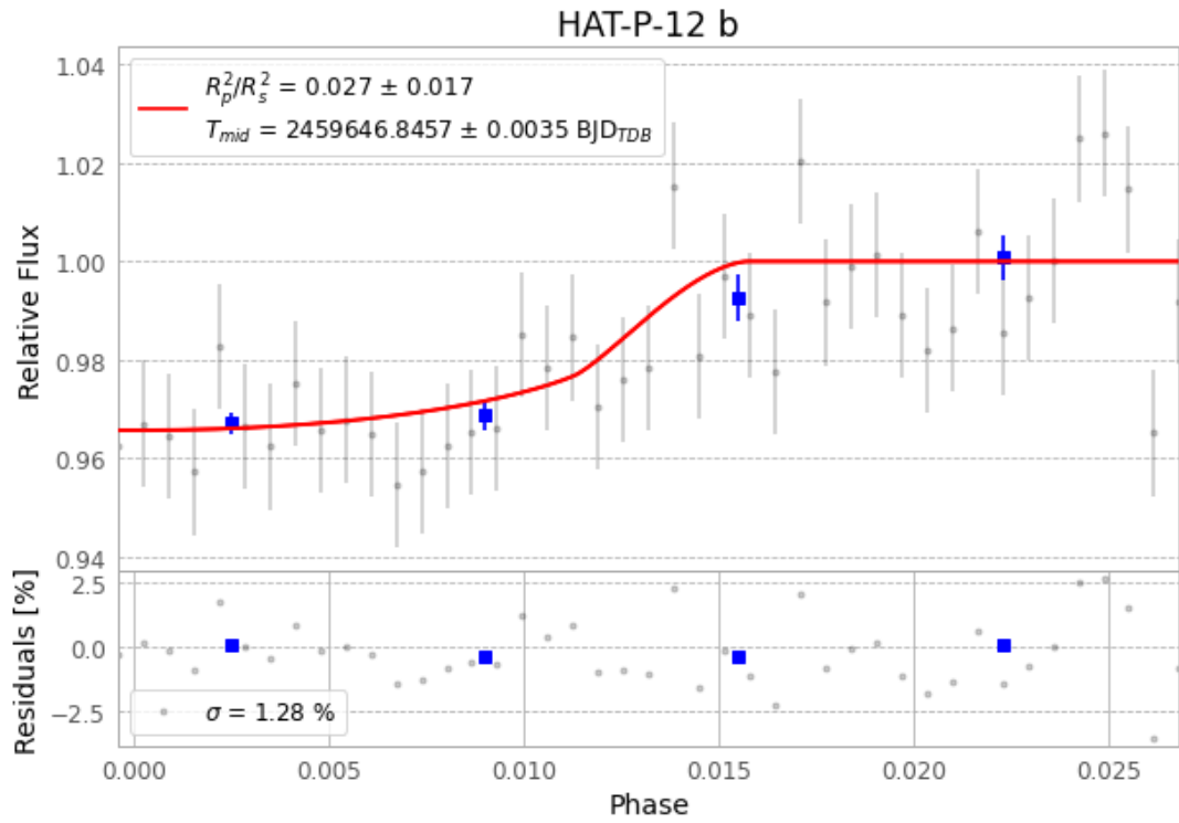
Figure 1 — FinalLightCurve_HAT-P-12 b_2022-03-08.png (SHA-256 566d7e88037e4df0...)
