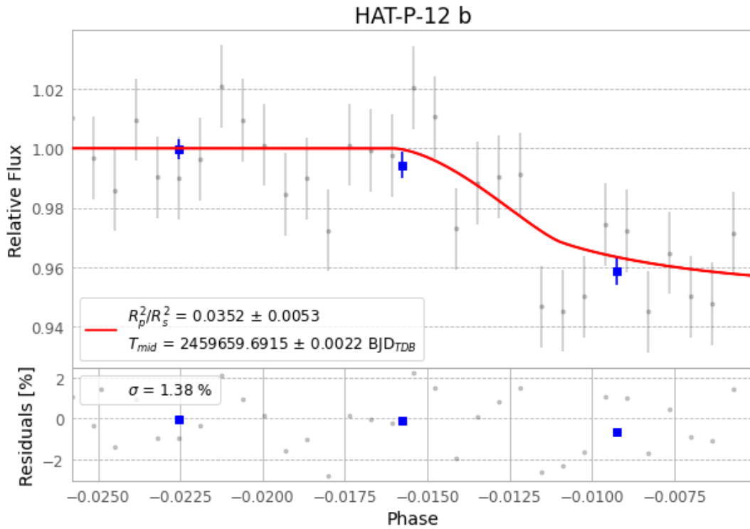
Figure 1 — FinalLightCurve_HAT-P-12 b_2022-03-24.png (SHA-256 cce11329c49b1ed4...)
